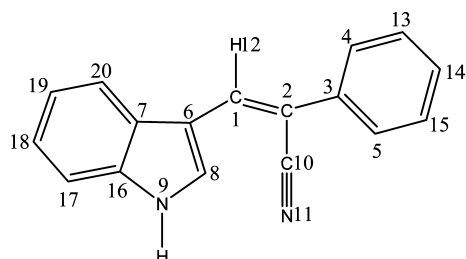
Scheme 1. Structure of 3-(2-Cyano-2-phenylethenyl-Z)-NH-indole Molecule
