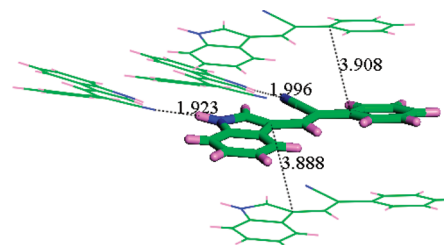
Figure 2. Close look at the molecular packing structure.
