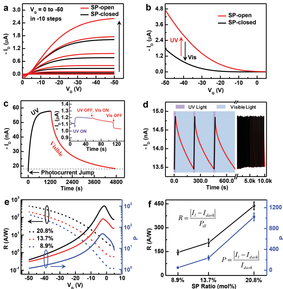
Figure 2. Photoresponsive characteristics of pentacene OFETs with SP-co-MMA gate dielectrics. a) Output and b) transfer properties of a SP-co-MMA-3 device before and after UV irradiation. V_D = -50 V. c) Temporal evolution of I_D with one complete cycle, V_D = -30 V and V_G = -15 V. The inset shows the time evolution of I_D for a control device with PMMA dielectrics, which does not contain SP units, under UV (365 nm) and visible ( \lambda > 520 nm) irradiation. V_D = -30 V and V_G = -15 V. d) Time evolution of I_D for the same device over a period of \approx 3 h with the first three cycles expanded for clarity, indicating reversible photoswitching modulation under UV and visible irradiation. V_D = -30 V and V_G = -15 V. e) Responsivity ( R ) and photosensitivity ( P ) values with the evolution of V_G for SP-co-MMA devices with three different molar percentages of SP units. V_D = -50 V and the irradiance power is 7.4 \mu\text{W cm}^{-2} . f) Both R and P values increase with increasing molar percentages of SP units (10 devices for each SP ratio).
