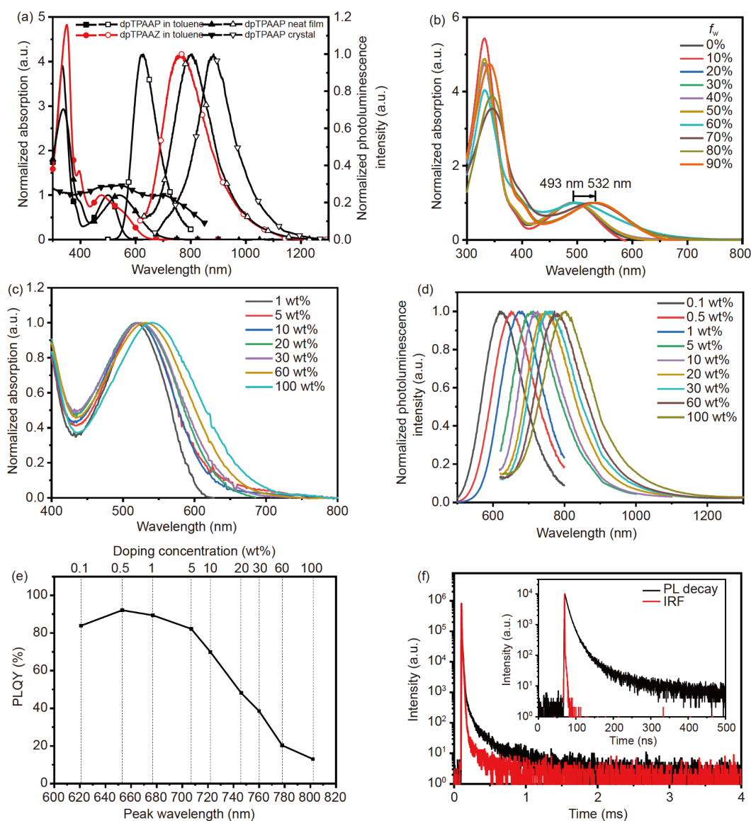
Figure 3 (a) Absorption (solid symbol) and PL (open symbol) spectra of dpTPAAP and dpTPAAZ in toluene ( 1 \times 10^{-5} mol L -1 ), dpTPAAP in neat films and single crystals. (b) Absorption spectra of dpTPAAP in THF/water mixtures ( 1 \times 10^{-5} mol L -1 ) with different water fractions ( f_w ). (c) Absorption spectra, (d) PL spectra and (e) PLQY of dpTPAAP in solid films with TPBi as a host at various doping concentrations at room temperature. (f) Transient PL decay curves of 30 wt.% dpTPAAP:TPBi films. Inset: the prompt decay curves in nanosecond scale (color online).
