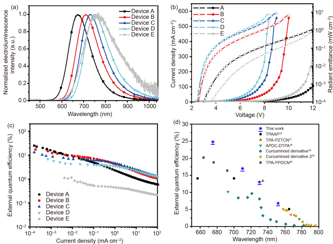
Figure 7 (a) Electroluminescence spectra recorded at the current of 1 \text{ mA cm}^{-2} for device A, B, C, D and E. (b) Current density-voltage-radiant emittance characteristics for device A, B, C, D and E. (c) EQE as a function of current density. (d) Maximum EQE summary of the representative deep-red and NIR OLEDs based on TADF emitters with emission peaks from 650 to 800 nm (color online).
